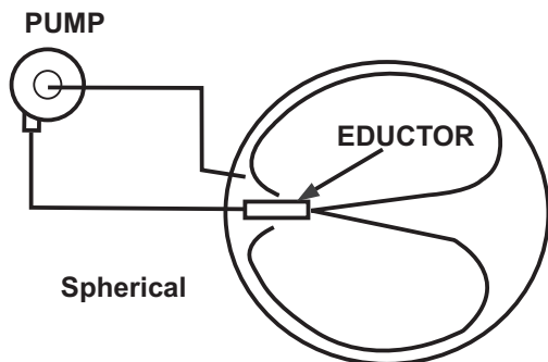
Figure 1 Educator in a round tank
