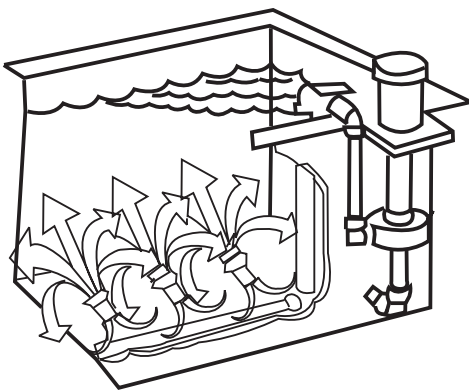
Figure 3 Multiple educator assembly
